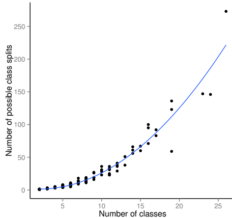
Fig. 3: Number of possible splits under a random-pair selection method vs number of classes for a number of UCI datasets. Logistic regression is used as the base learner.
