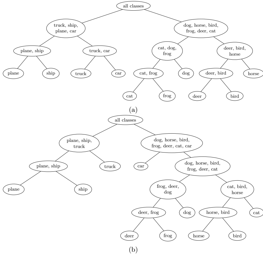
Fig. 6: Nested dichotomies trained on CIFAR-10, with (a) random-pair selection, and (b) centroid-based selection.
